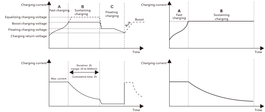
Fig. 1-5 SLD Battery charging stages diagram
