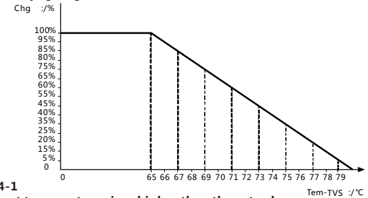
Fig. 4-1 When the ambient temperature rises higher than the set value, the controller will stop charging and discharging.
